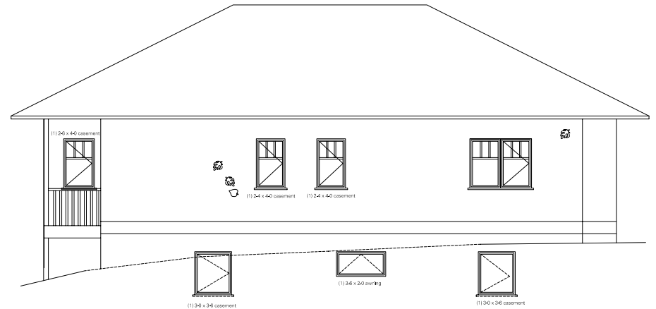
North elevation
