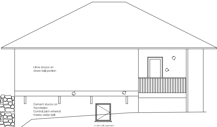
East elevation
